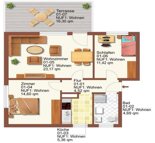
Erdgeschoss links
